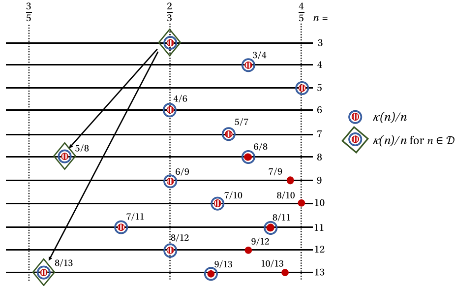
FIGURE 6. Construction of k[n] and \mathcal{D} in Theorem 2 for m=2 . Dots correspond to \frac{k}{n} s; circled dots correspond to \frac{k}{n} for k \in k[n] ; circled-striped dots correspond to \frac{\kappa(n)}{n} ; dots circumscribed by diamonds correspond to \frac{\kappa(n)}{n} for n \in \mathcal{D} . Arrows point in the direction of domination in the set \mathcal{D} .
